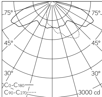
LED 3000 K 25.5 W 3756 lm-h = 7 m / CIE Flux 35 69 94 100 100 / A30 selon DIN 5...
