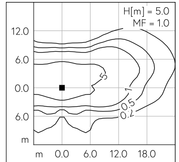
LED 3000 K 13.5 W 1895 lm-h H = 5 m / CIE Flux 35 67 94 100 100 / A30 selon DIN ...
