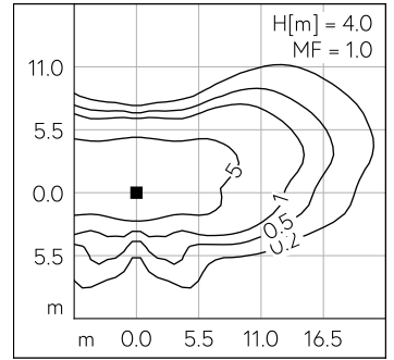
LED 3000 K 13.5 W 1895 lm-h H = 4 m / CIE Flux 35 67 94 100 100 / A30 selon DIN ...
