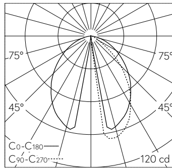
LED 3000 K 2.7 W 155 lm-h / CIE Flux 59 88 98 100 100 / A50 selon DIN 5040
