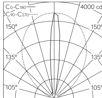
LED 4000 K 15.5 W 1379 lm-h / CIE Flux 0 0 4 0 100 / E84 selon DIN 5040
