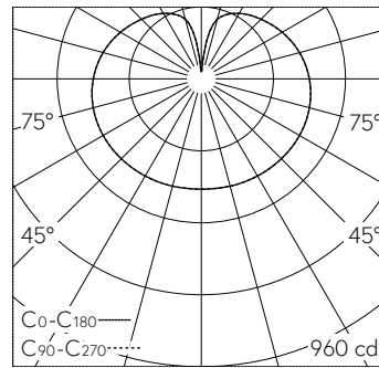
LED 4000 K 39,5 W 4240 lm-h / CIE Flux 25 50 75 55 100 / C12 selon DIN 5040
