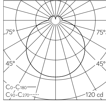
LED 4000 K 3,0 W 351 lm-h / CIE Flux 41 71 90 84 100 / B32 selon DIN 5040
