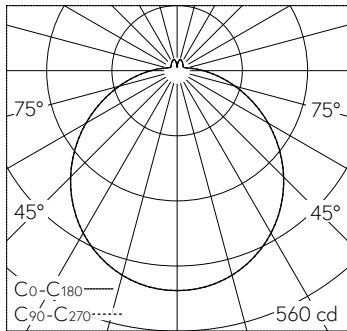
LED 3000 K 21 W 1645 lm-h / CIE Flux 43 73 90 91 100 / A31 selon DIN 5040
