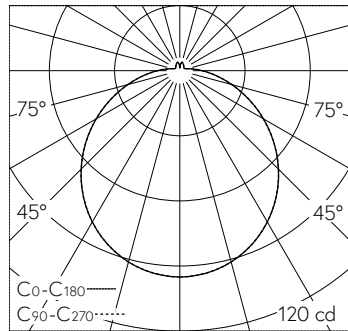
LED 3000 K 3,0 W 319 lm-h / CIE Flux 43 73 91 93 100 / A31 selon DIN 5040
