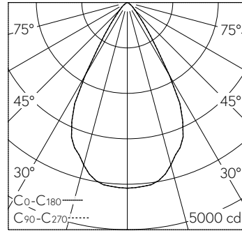
LED 3000 K 29 W 3585 lm-h 58° 13165M / CIE Flux 93 99 100 100 100 / A80 selon ...
