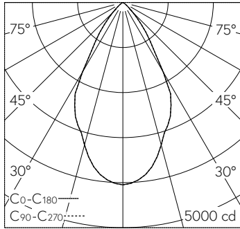
LED 3000 K 29 W 3426 lm-h 58° / CIE Flux 92 100 100 100 100 / A80 selon DIN 5040
