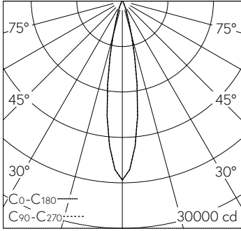
LED 3000 K 29 W 3516 lm-h 19.4° / CIE Flux 97 100 100 100 100 / A80 selon DIN 50...
