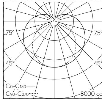
LED 3000 K 218 W 23820 lm-h / CIE Flux 36 64 84 79 100 / B31 selon DIN 5040
