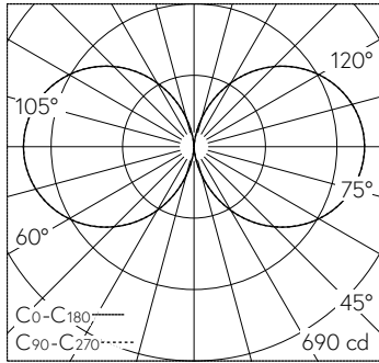
LED 3000 K 58 W 5220 lm-h / CIE Flux 13 37 66 50 100 / C11 selon DIN 5040
