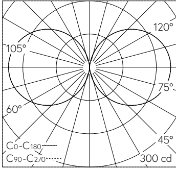
LED 4000 K 30 W 2309 lm-h / CIE Flux 13 37 66 50 100 / C11 selon DIN 5040
