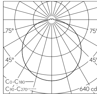
LED 3000 K 22.2 W 2003 lm-h 116° / CIE Flux 45 75 93 95 100 / A41 selon DIN 5040
