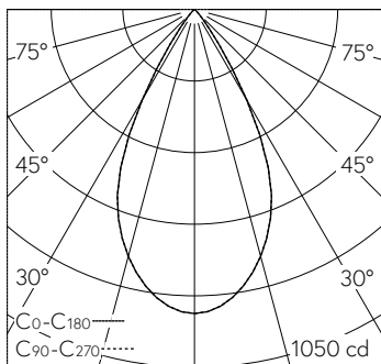
LED 4000 K 7.5 W 619 lm-h 54° / CIE Flux 98 100 100 100 100 / A80 selon DIN 5040
