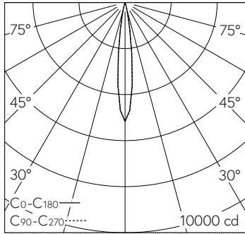
LED 4000 K 7.5 W 619 lm-h 13.6° / CIE Flux 100 100 100 100 100 / A80 selon DIN 5...
