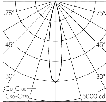
LED 4000 K 7.5 W 459 lm-h 18.0° / CIE Flux 100 100 100 100 100 / A80 selon DIN 5...
