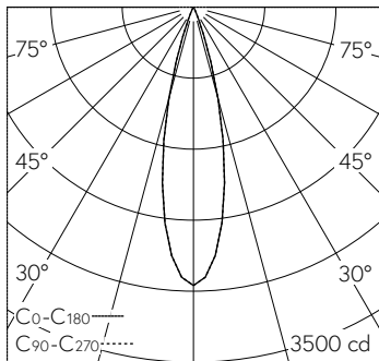
LED 4000 K 7.5 W 511 lm-h 24° / CIE Flux 100 100 100 100 100 / A80 selon DIN 5040
