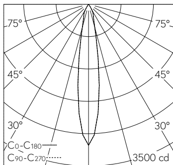
LED 4000 K 4.9 W 483 lm-h 17.2° / CIE Flux 100 100 100 100 100 / A80 selon DIN 5...
