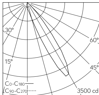
LED 4000 K 4.9 W 430 lm-h 30° / CIE Flux 93 100 100 100 100 / A80 selon DIN 5040
