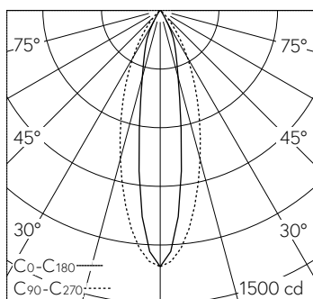
LED 4000 K 4.9 W 415 lm-h 19.0°/36° B10013 / CIE Flux 96 100 100 100 100 / A80 s...
