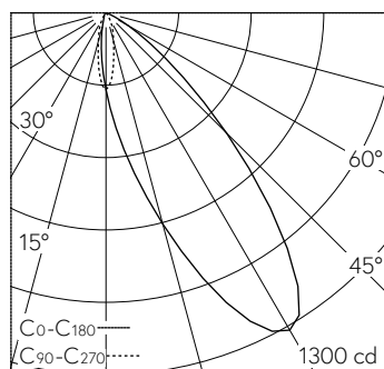
LED 4000 K 4.9 W 360 lm-h 30° B10013 / CIE Flux 81 99 100 100 100 / A70 selon DI...
