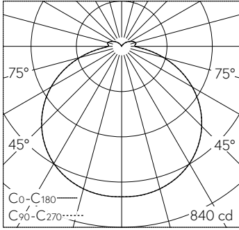
LED 3000 K 28.5 W 2745 lm-h / CIE Flux 42 73 92 90 100 / A31 selon DIN 5040
