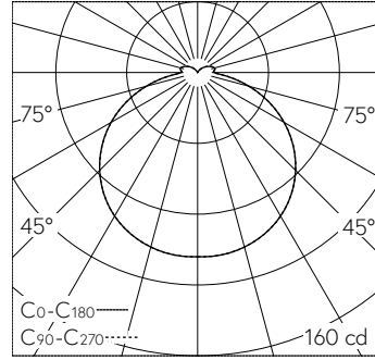
LED 3000 K 3,0 W 389 lm-h / CIE Flux 42 73 92 90 100 / A31 selon DIN 5040
