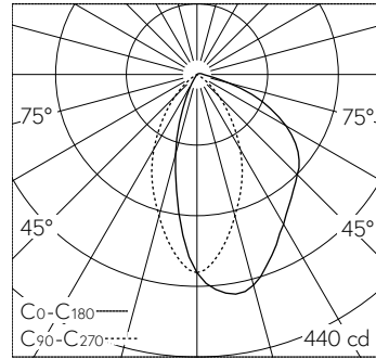
LED 4000 K 3,0 W 382 lm-h / CIE Flux 61 86 97 99 100 / A50 selon DIN 5040
