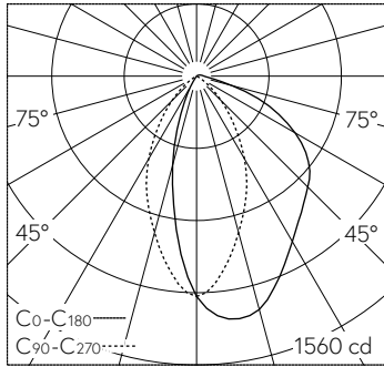
LED 3000 K 19 W 1466 lm-h / CIE Flux 61 85 97 99 100 / A50 selon DIN 5040
