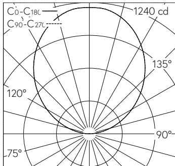
LED 3000 K 33 W 3190 lm-h / CIE Flux 0 0 0 0 100 / E03 selon DIN 5040
