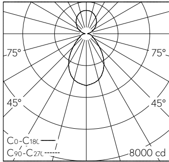
LED 3000 K 90 W 9904 lm-h / CIE Flux 61 84 94 60 100 / B53 selon DIN 5040
