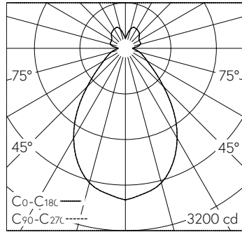
LED 3000 K 90 W 9904 lm-h / CIE Flux 61 83 94 73 100 / B52 selon DIN 5040
