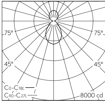
LED 3000 K 68 W 7112 lm-h / CIE Flux 61 84 94 60 100 / B53 selon DIN 5040
