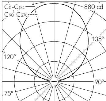
LED 3000 K 25 W 2291 lm-h / CIE Flux 0 0 0 0 100 / E03 selon DIN 5040
