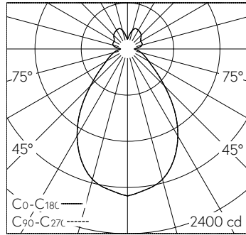
LED 3000 K 68 W 7112 lm-h / CIE Flux 61 83 94 73 100 / B52 selon DIN 5040
