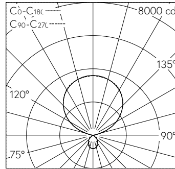
LED 2700 – 6500 K 83 W 11595 lm-h / CIE Flux 66 92 98 12 100 / D63 selon DIN 5040
