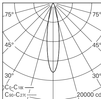
LED 3000 K 36 W 2572 lm-h 20° / CIE Flux 98 100 100 100 100 / A80 selon DIN 5040
