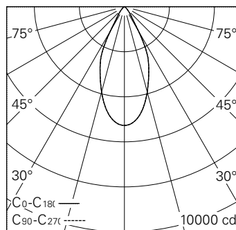
LED 4000 K 27 W 3242 lm-h 48° / CIE Flux 94 99 100 100 100 / A80 selon DIN 5040
