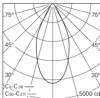
LED 3000 K 27 W 2574 lm-h 48° / CIE Flux 94 99 100 100 100 / A80 selon DIN 5040
